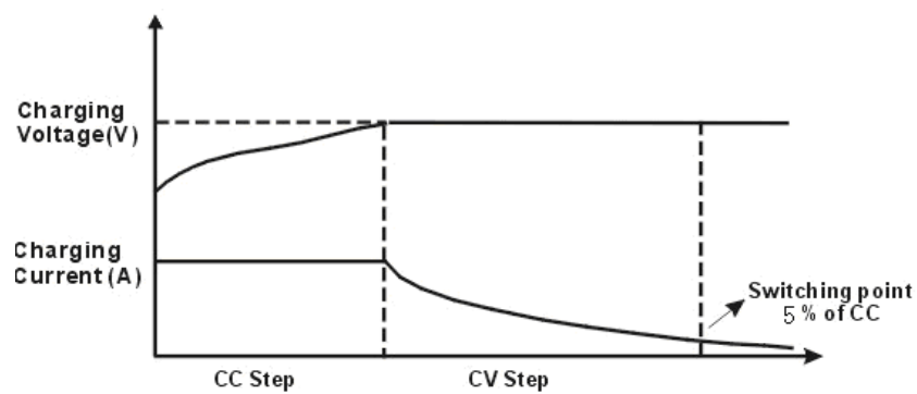
Charging Curve
